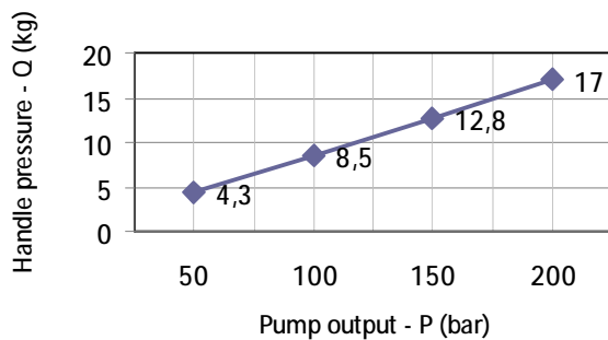
HP-10 Hand Pump Pump yield
