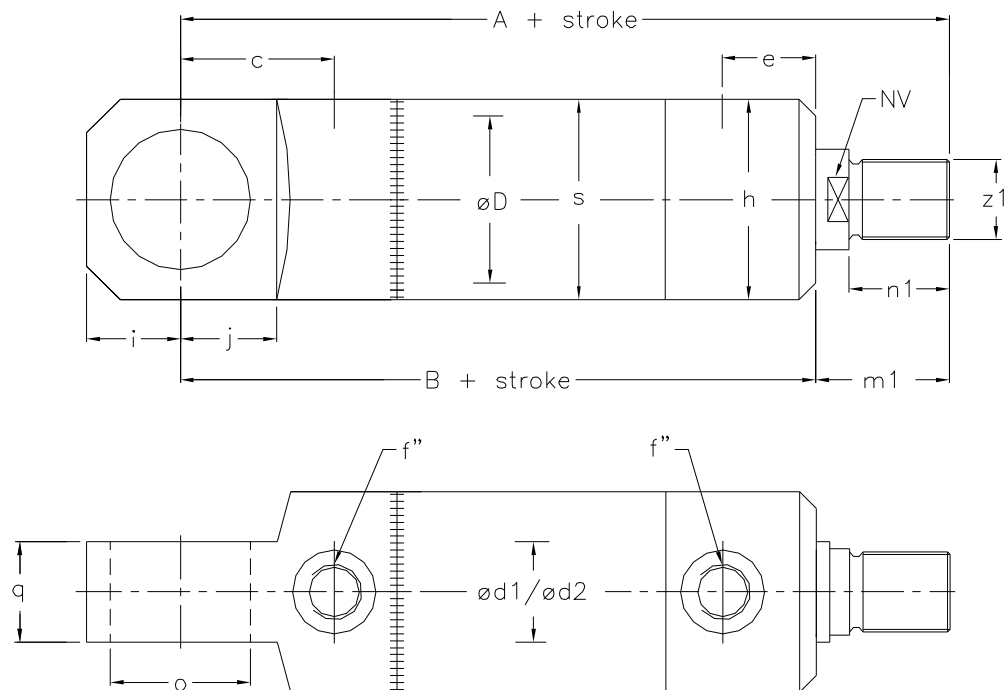
Dimension table
